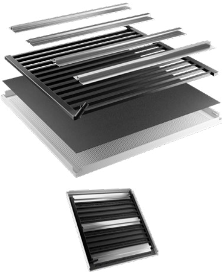
1. Heat conducting plates 2. Heating and cooling grid 3. Acoustic fleece 4. Metal cassette
